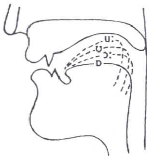
Fig. 9 Tongue positions for /u:/, /ʊ:/, /ɔ:/, /ɒ/
